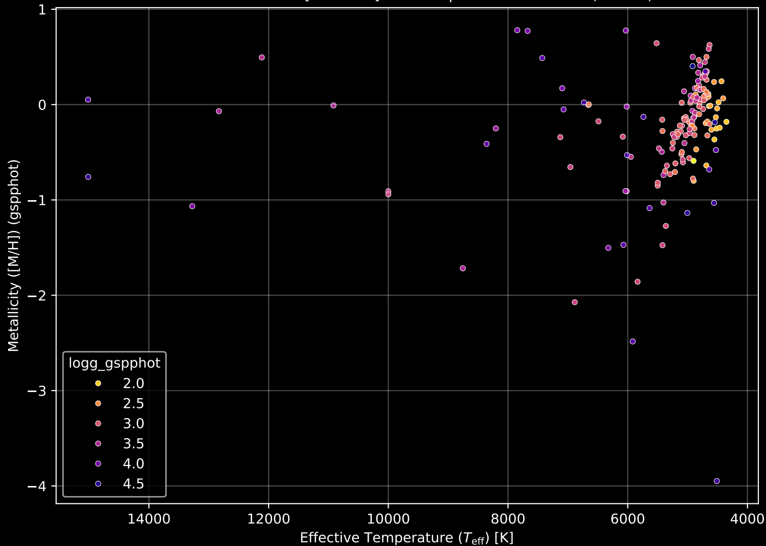
APOGEE DR17 Field: [002-02-O] Stellar Population Parameters (n= 166)
