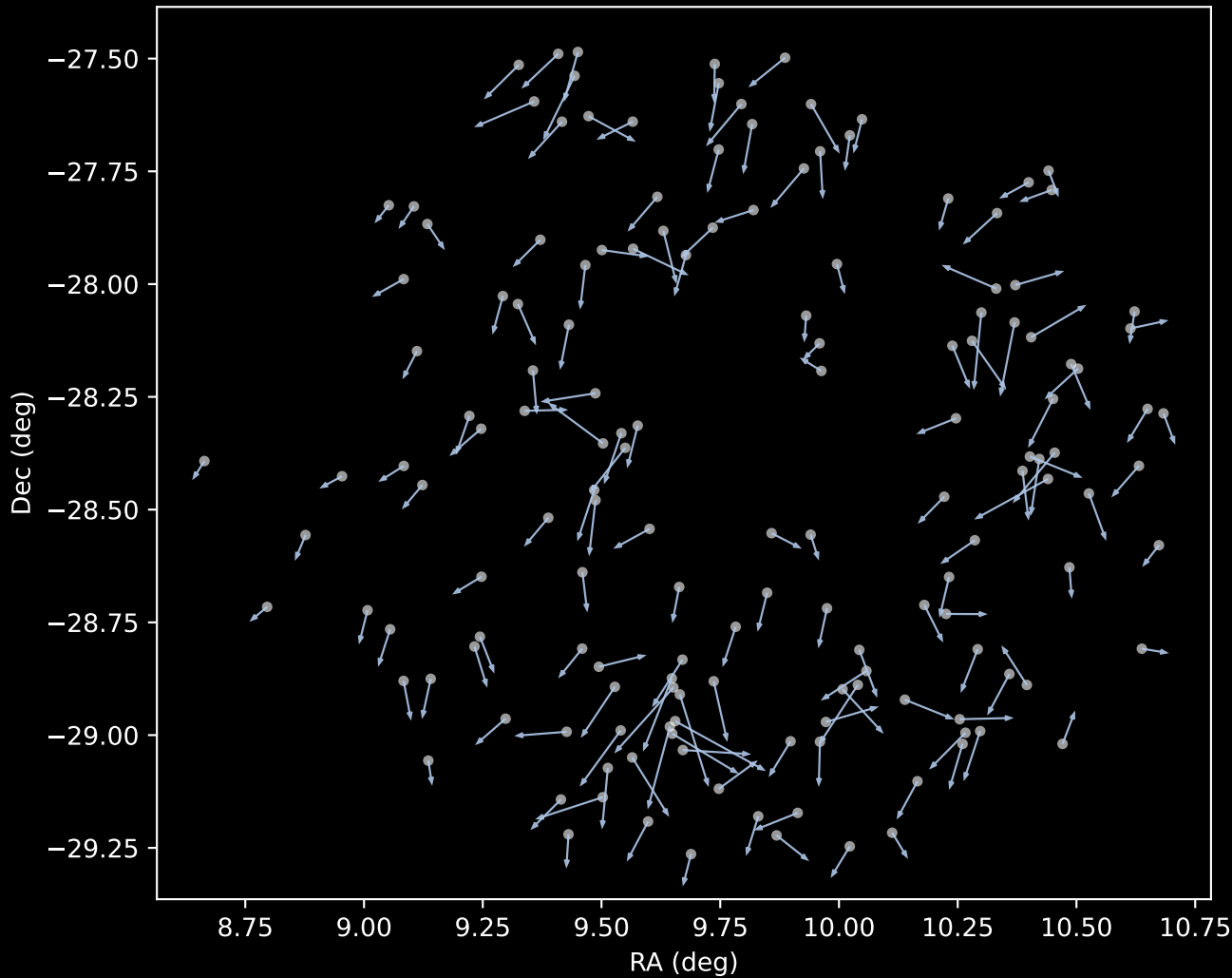
APOGEE DR17 Cluster 1 Proper Motion Vectors (n=154)
