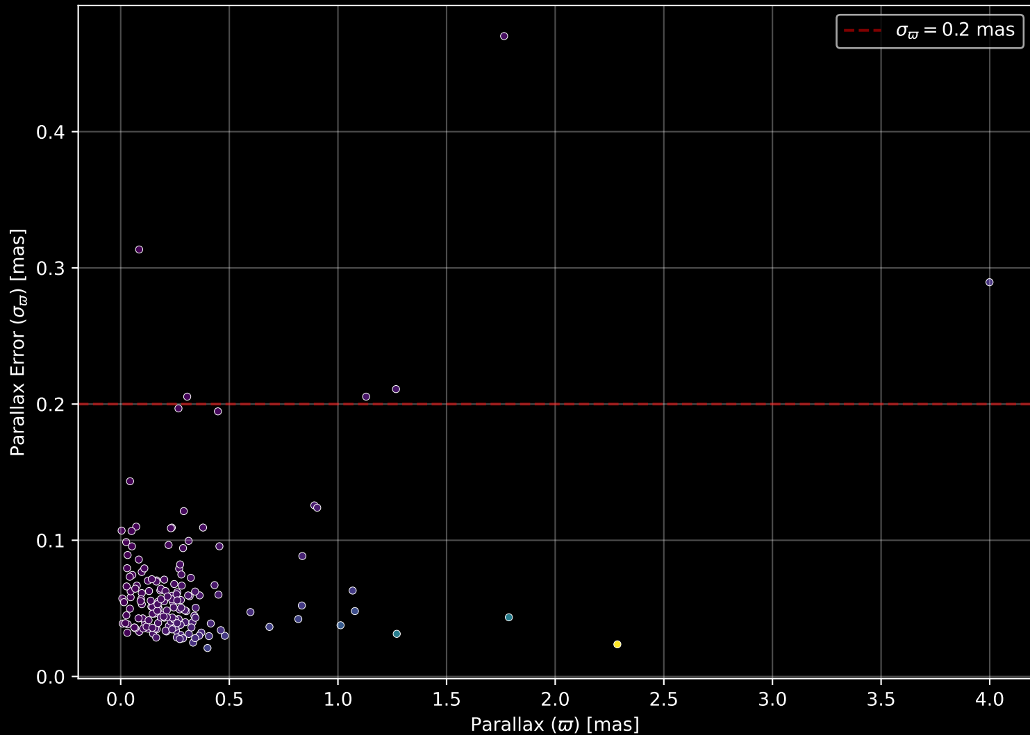
APOGEE DR17 Field: [002-02-O] Parallax Quality (n= 166)
