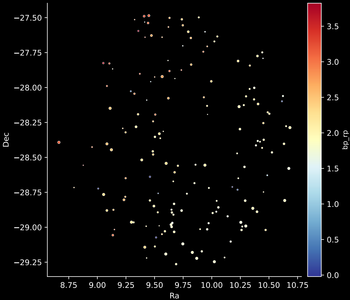
APOGEE DR17 Field: [002-02-O] Stars: 166
