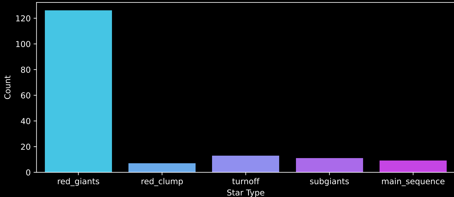
APOGEE DR17 Field: [002-02-O] Count plot of Star Type
