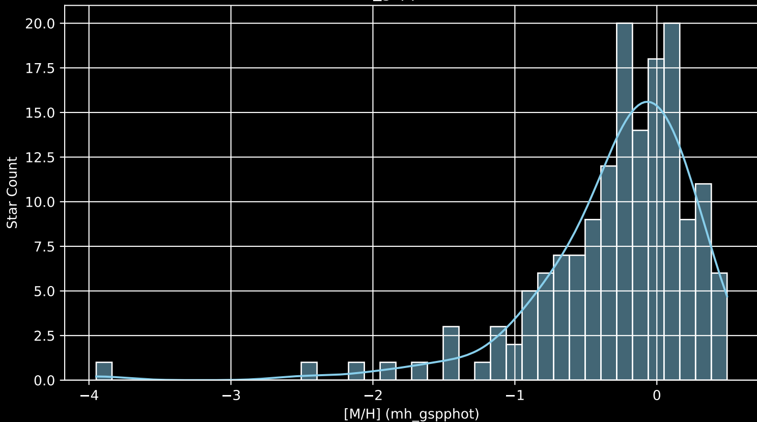
APOGEE DR17 Field: [002-02-O] [M/H] (mh_gspphot) (n= 158)
