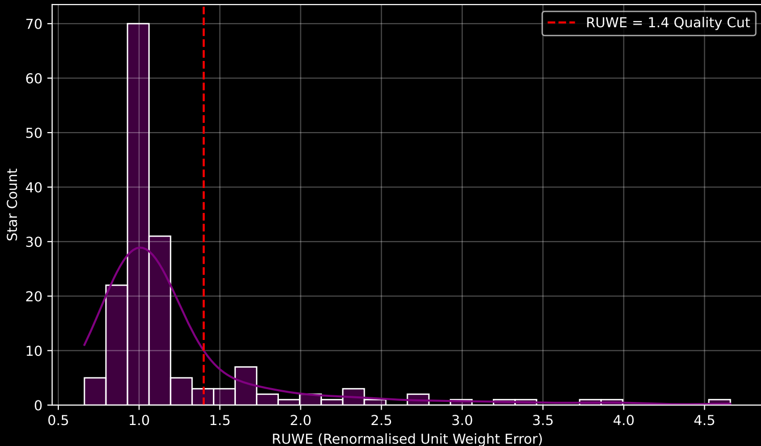
GAPOGEE DR17 Field [002-02-O] RUWE Distribution (n= 164)
