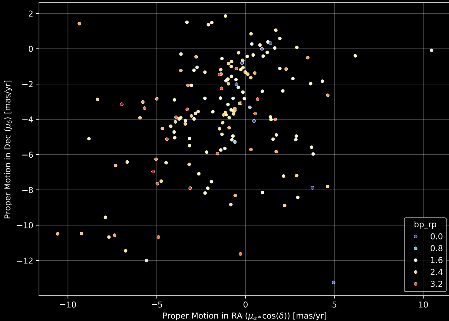
APOGEE DR17 Field: [002-02-O] Proper Motion Diagram (n= 166)
