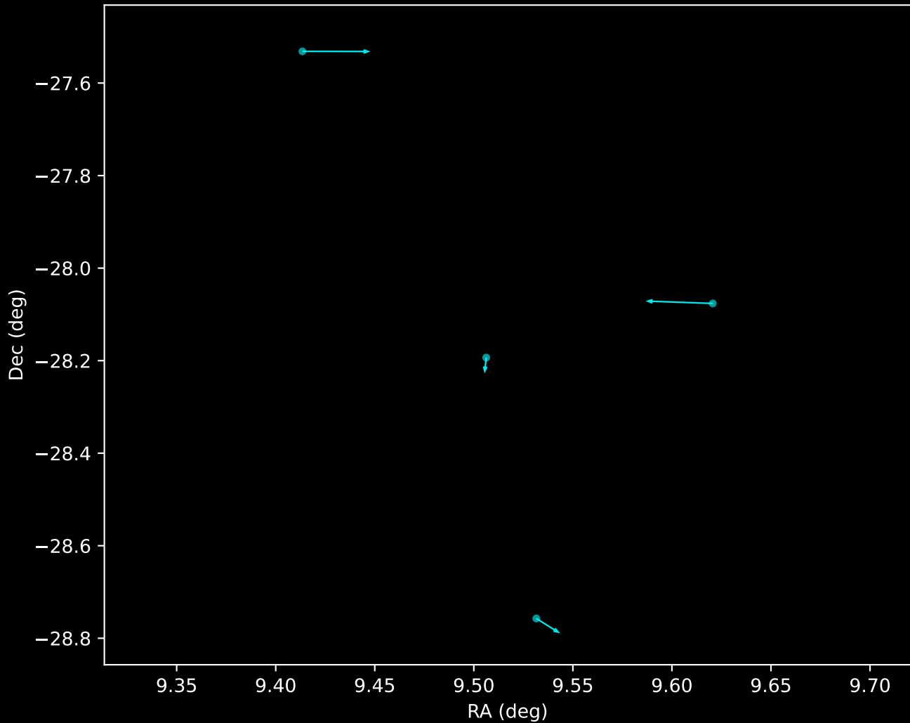
APOGEE DR17 Noise Stream Proper Motion Vectors (n=4)
